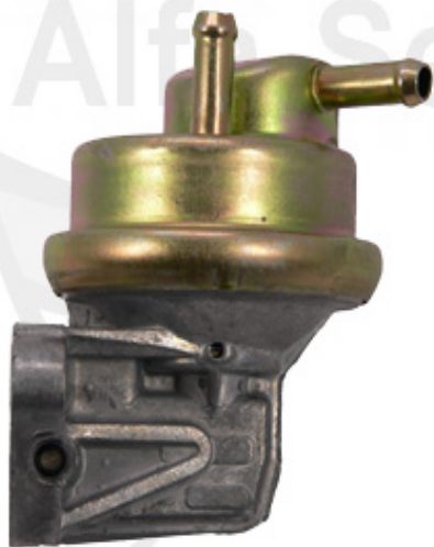
1. KP 0565 Vergaser/carburetor
